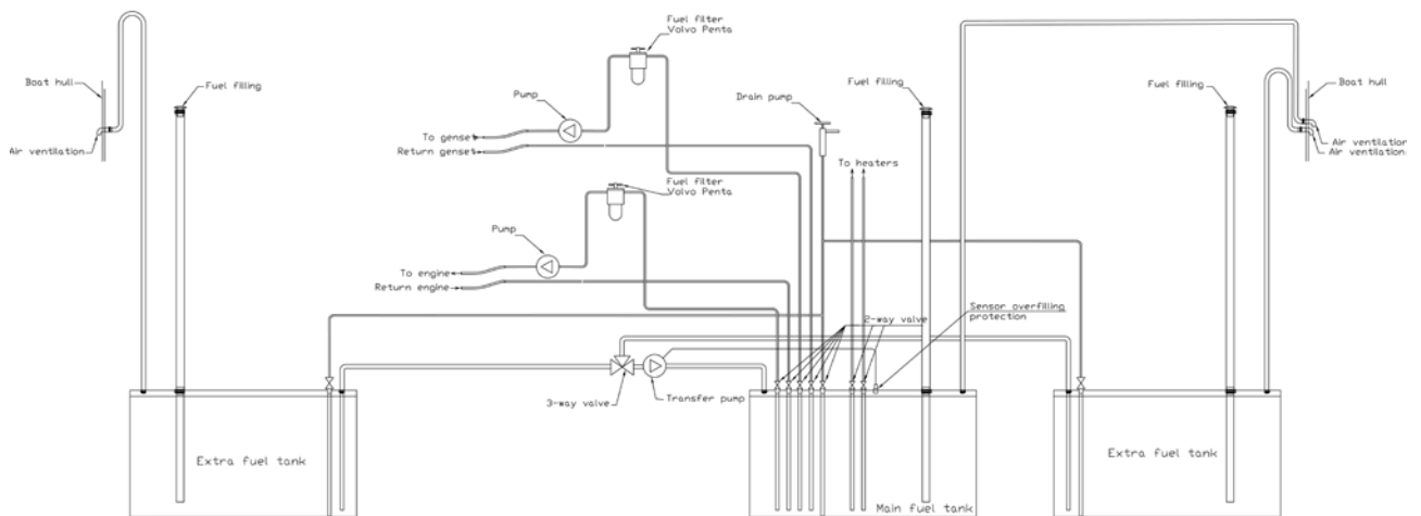
Principle drawing Diesel system HR 57
